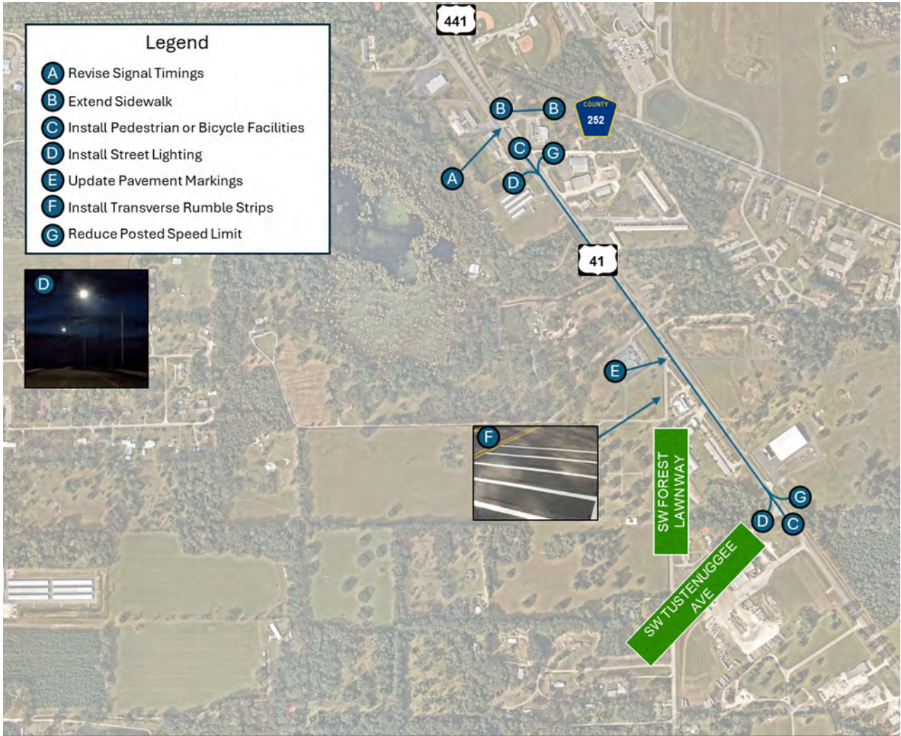
Figure 52: Proposed Countermeasures, Priority 9
