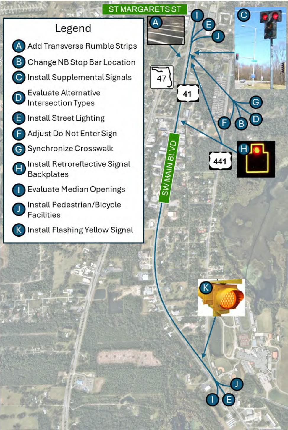
Map 38: Proposed Counter measures, Priority 12
